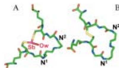
Figure 3. A) Structure for SbT(S) 2 which is consistent with the observed NMR rOe; B) crystal structure of the disulfide form of trypanothione from a complex of trypanothione reductase and trypanothione. [11] All hydrogen atoms are omitted for clarity. C, green; N, blue; O, red; S, yellow; Sb, purple.
