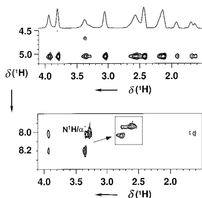
Figure 2. Expansion of the 200 ms 2D ROESY NMR spectra of SbT(S) 2 at 278 K (pH 7.4). A variety of cross-peaks were observed between water protons and the hydrophobic part of spermidine, the \alpha - and \beta -protons of Cys, and the \alpha -protons of Gly (top); a section through the 2D ROESY spectrum at the chemical shift of water is plotted above the spectrum. A weak long-range rOe between N 1 H and \alpha' -CH 2 was clearly observed (bottom).
